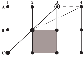
Figure 5: Tie Breaking and the Triangle Inequality
